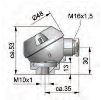
Form D - LA / shape D - LA
