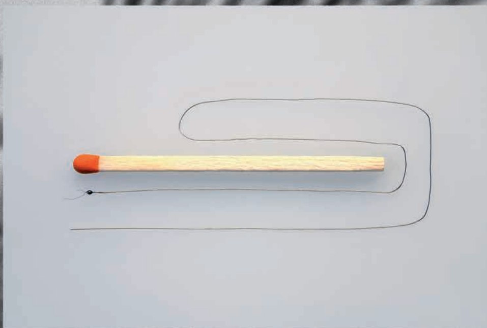
mineral insulated thermocouple Ø 0,15 mm with insulated hot junction
